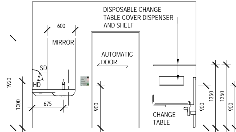
ELEVATION C
