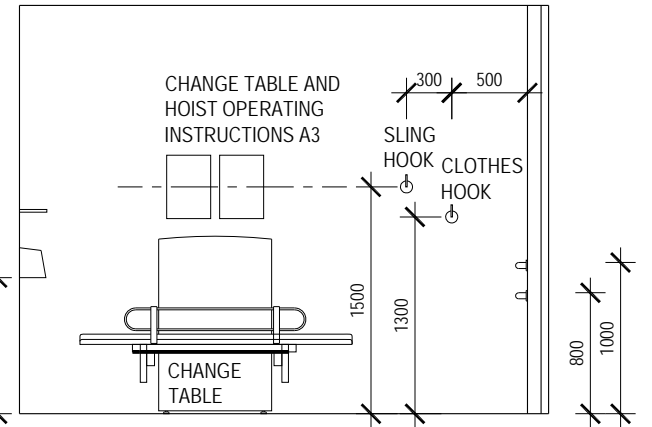
ELEVATION D
